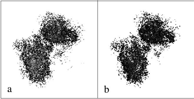
Fig. 2. Spatial variation of the extinction and ionization across N 159-5. a) The H\alpha/H\beta ratio varies between 5 and 10 corresponding to a visual extinction between 1.5 and 3.5 mag. b) The [O\ III] \lambda 5007/H\beta varies between 3.5 and 8. The field size and orientation of both frames are identical to the inset of Fig. 1.
