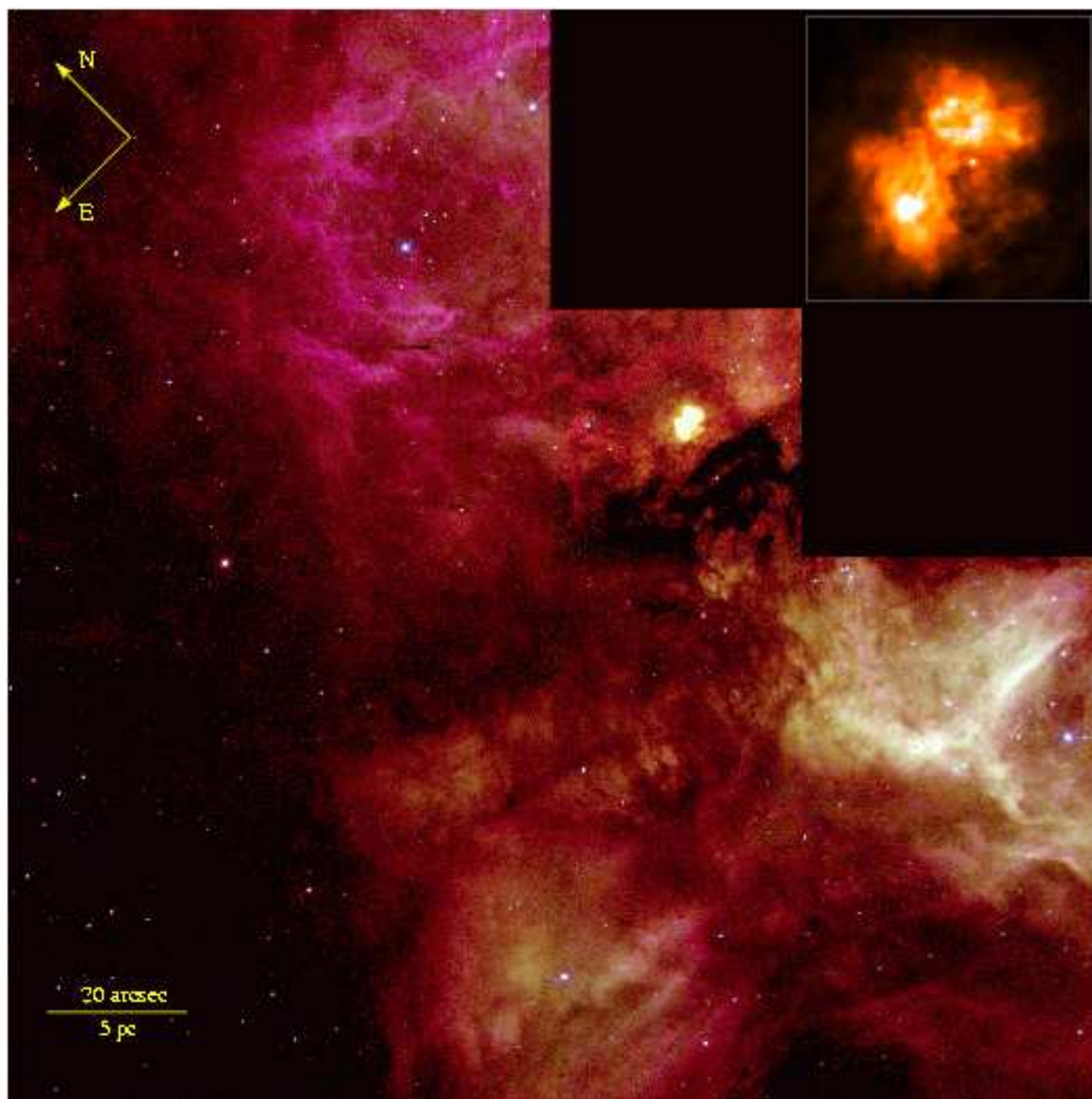
Fig. 1. A “true color” composite image of the LMC H II region N 159 as seen by WFPC2, based on images taken with filters H\alpha (red), [O III] (green), and H\beta (blue). The N 159-5 “blob” is the high excitation compact object lying in the center of the smaller PC frame. Note how the hardness of the radiation field varies from north to south across the image. The yellowish colors represent higher excitation gas as traced by the [O III] emission line and are mainly found in the giant ridge in the southern part of N 159 and in the blob. In the northern part the emission is principally due to relatively lower energy H\alpha photons. inset: A false color image of N 159-5 in H\alpha showing the internal morphology of the butterfly-shaped H II region. Field size \sim 5'' \times 5'' ( 1.3 \times 1.3 pc).
