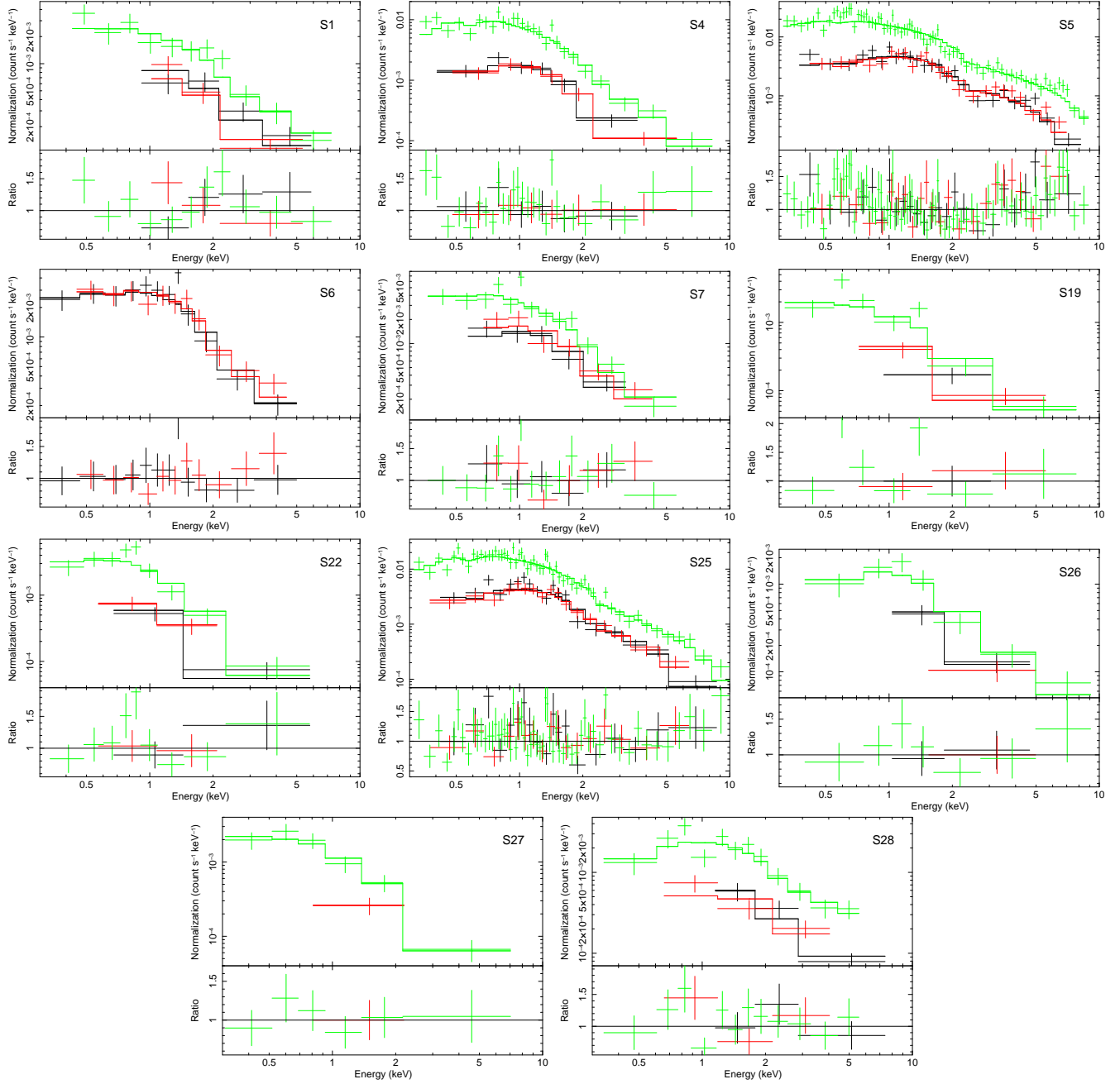
Figure 5. XMM-Newton EPIC spectra of the 11 sources with > 100 net PN or MOS counts. PN data points and power-law+absorption models are shown in green; those of the MOS data are shown in red/black.
