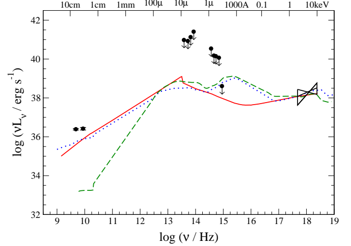
Figure 11. The spectral energy distribution (SED) of the nuclear source in NGC 1672. The IR and optical measurements are shown as upper limits, since there is likely to be contamination from starlight at these wavelengths. Also plotted is the average LLAGN SED of Ho (2005) ( solid red line ), and the average radio-loud ( dotted blue line ) and radio-quiet ( dashed green line ) quasar SEDs of Elvis et al. (1994), normalized to the X-ray luminosity of NGC 1672 at 2 keV.
