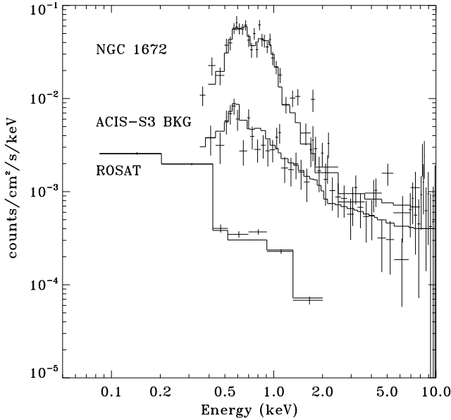
Figure 7. The Chandra ACIS spectral data and fit for the diffuse galaxy spectrum, the Galactic foreground/extragalactic background, and the ROSAT All-Sky Survey (RASS) data. The ACIS-S1 background spectrum is not shown for clarity.
