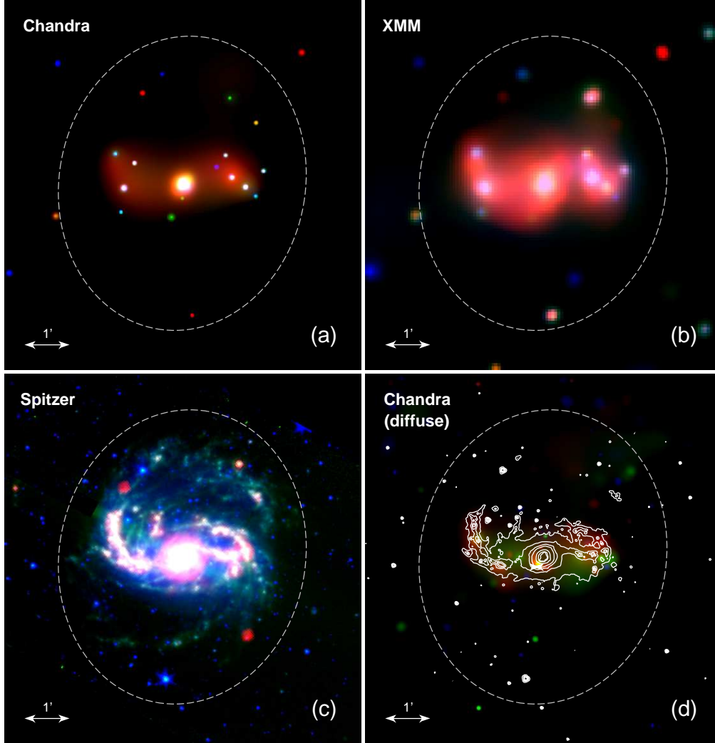
Figure 2. (a) Chandra 3-color ACIS-S image of NGC 1672: red = 0.3–1 keV, green = 1–2 keV, blue = 2–10 keV. (b) XMM-Newton EPIC (MOS1+MOS2+PN) 3-color image (in the same energy bands). (c) Spitzer 3-color image: red = 24\mu\text{m} (MIPS), green = 8\mu\text{m} (IRAC), blue = 3.6\mu\text{m} (IRAC). (d) Chandra 3-color image of the diffuse X-ray emission. Contours from the Spitzer IRAC stellar-continuum-subtracted 8\mu\text{m} data are overlaid, which are spatially correlated with the X-ray emission. The D_{25} ellipse of the galaxy is shown with a dashed white line. All images are on the same scale and co-aligned. North is up, east to the left.
