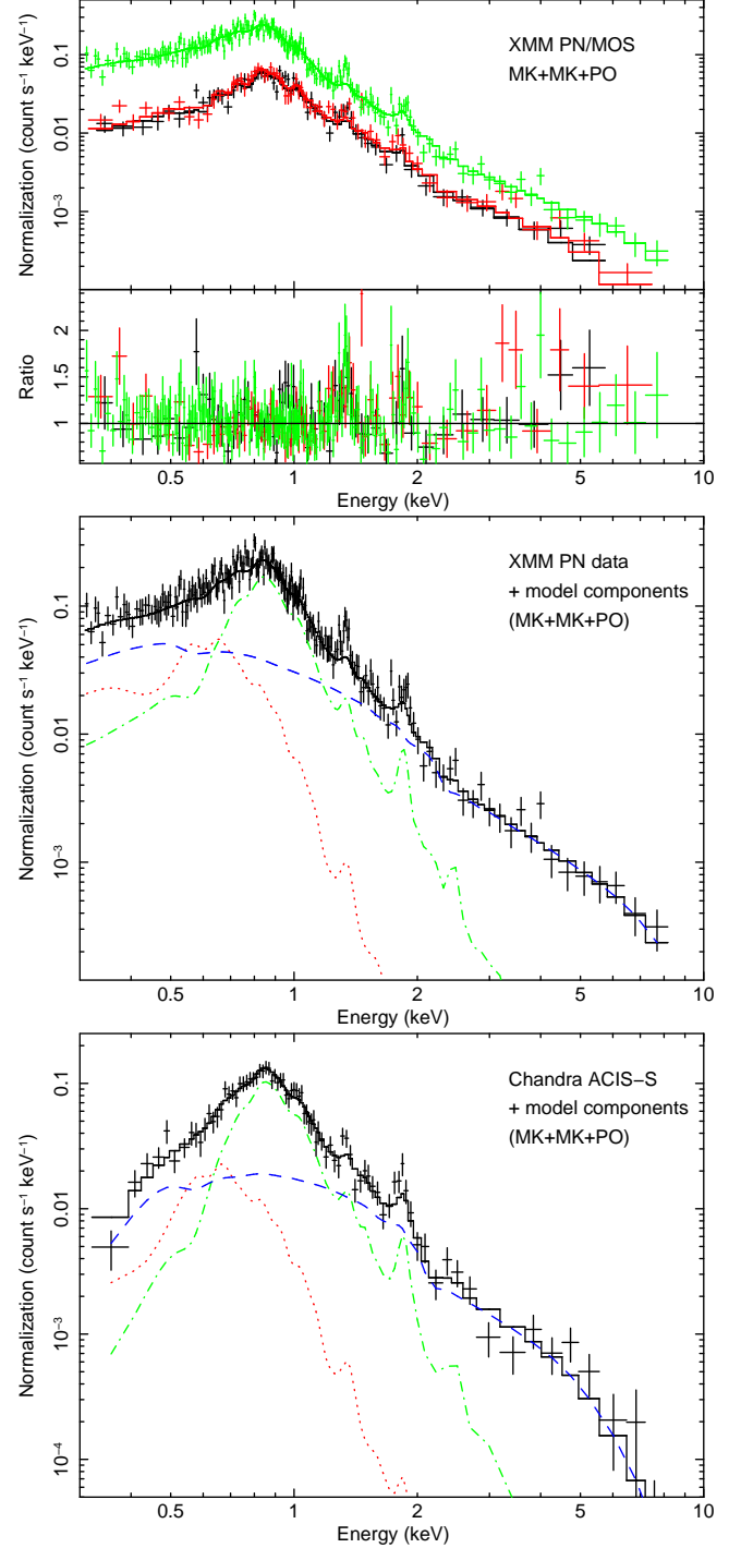
Figure 10. X-ray spectra from the central 22'' radius region of NGC 1672, which includes the nucleus and circumnuclear ring. Top: XMM-Newton folded model and PN (green) and MOS1/MOS2 (black/red) spectra. Middle: folded model and PN spectrum to illustrate the contributions from the model components, denoted by dashed blue (power-law), dotted red (cool MEKAL) and dot-dashed green (warm MEKAL) lines. Bottom: the ACIS-S spectrum with MK+MK+PO model.
