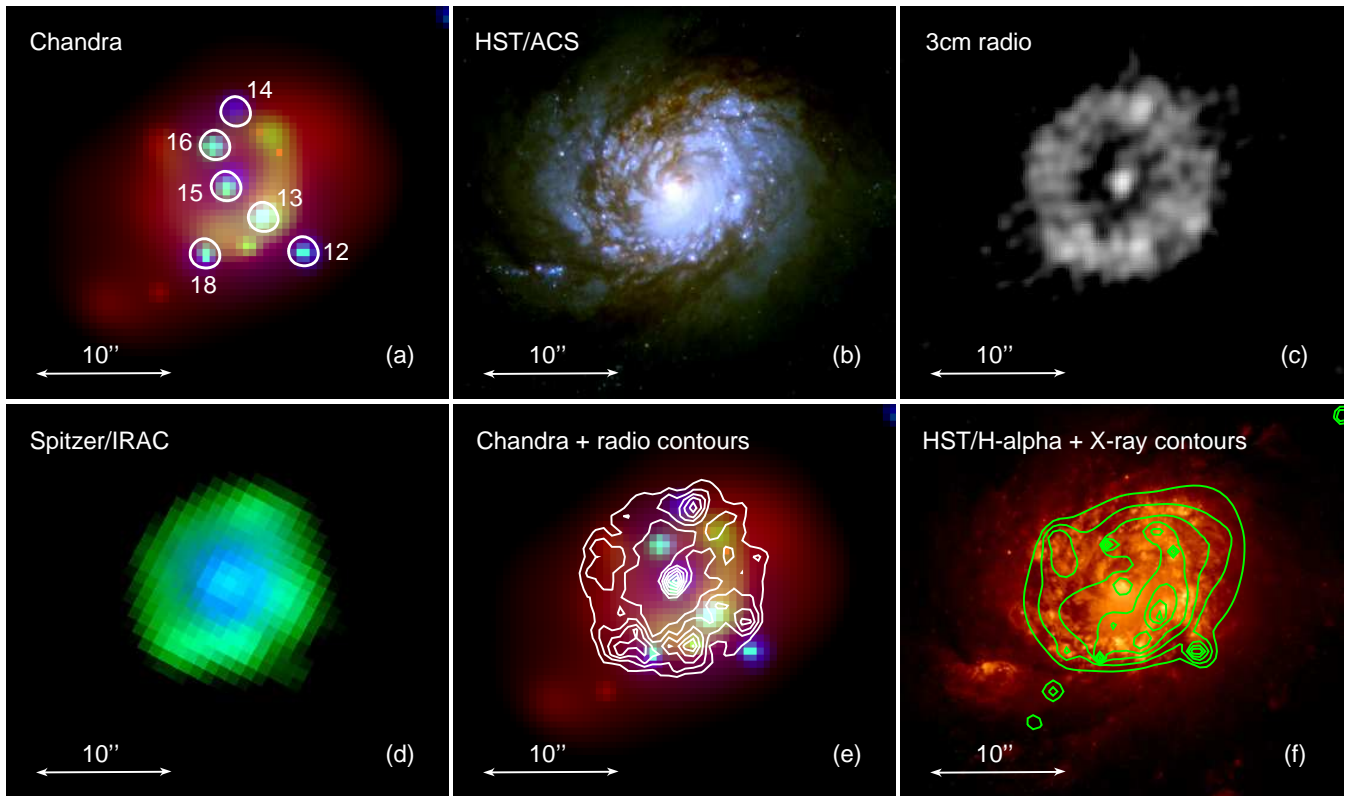
Figure 8. The circumnuclear region of NGC 1672. (a) Chandra 3-color image: red = 0.3–1 keV, green = 1–2 keV, blue = 2–10 keV. The circumnuclear ring is evident, surrounding a weak nuclear X-ray point source (#15). The white polygons denote the 90% extraction regions of the detected point sources. (b) HST/ACS 3-color image: red = combined F658N (H \alpha ) + F814W ( I ), green = F550M ( V ), blue = F435W ( B ). (c) 3-cm ATCA radio image. (d) Spitzer /IRAC 2-color image: green = 8 \mu m, blue = 3.6 \mu m. (e) Chandra 3-color image with ATCA 3-cm radio contours overlaid. (f) HST H \alpha image with Chandra broad-band (0.3–10 keV) contours overlaid. All images are on the same scale and co-aligned. North is up, east to the left.
