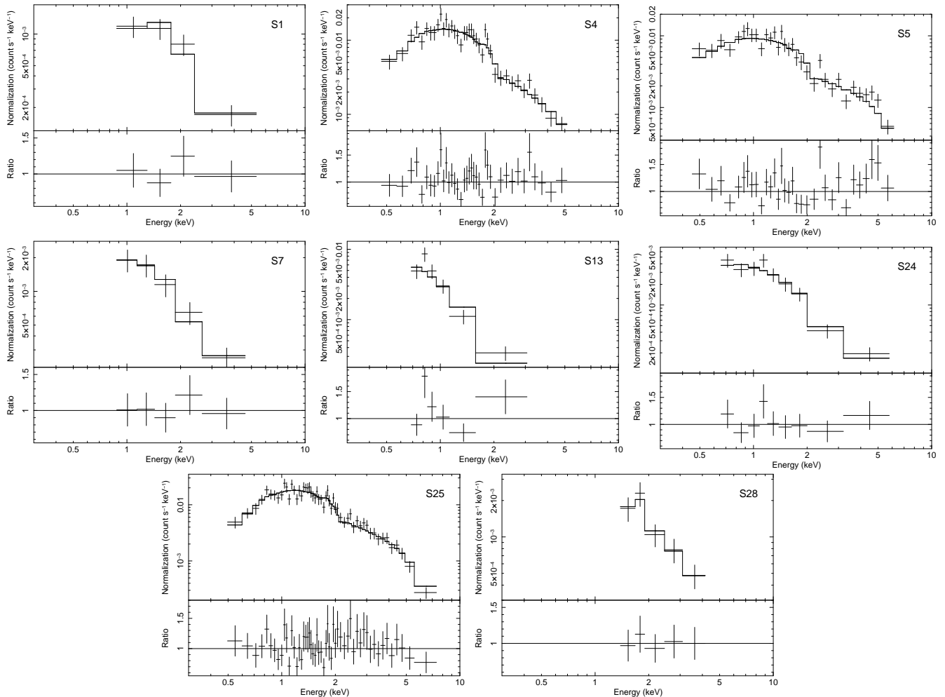
Figure 6. Chandra ACIS-S spectra of the 8 sources with > 100 net counts, together with the powerlaw+absorption models.
