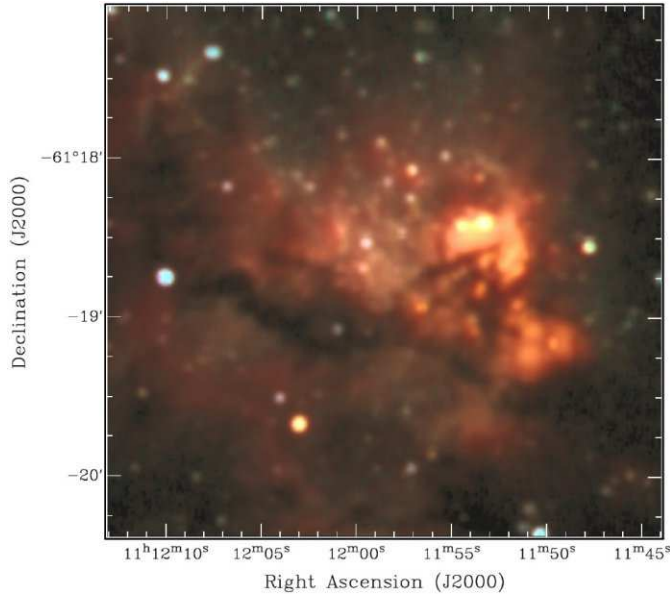
Fig. 3. HK_sL (Blue=H, Green= K_s , Red=L) composite colour image of RCW 57 created using 2MASS and SPIREX images. Regions bright in the L-band ( 3.5\mu\text{m} ) can be seen in red or orange, indicating the presence of young stellar objects. Prominent dust lanes are also apparent.
