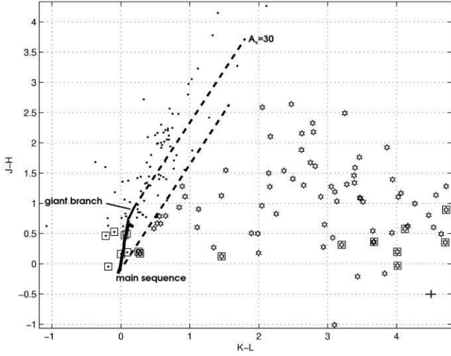
Fig. 7. JHK_sL colour-colour diagram for RCW 57. The thick solid line shows the position of the unreddened main sequence for spectral types O6-8 to M5. The thin solid line above shows the giant branch for spectral types K0 to M5 and extends from (J-H)=0.5 , (K_s-L)=0.07 to (J-H)=0.9 to (K_s-L)=0.19 . The dashed lines show the reddening vector up to A_V = 30 assuming an extinction law \propto \lambda^{-1.7} . Star shaped symbols are stars identified as having an IR-excess (§ 4.2). Sources in squares are have (J-K_s)<0.7 (see § 3.3). The cross in the lower right of the diagram indicates the mean errors for all stars. 209 stars lie above the 90% completeness limit and 75 of these lie outside the reddening band and are therefore considered to have IR-excess (Table 3 and 4).
