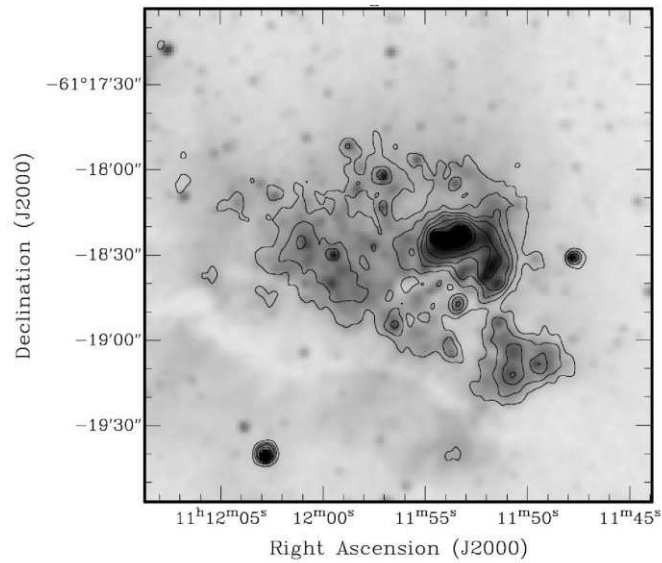
Fig. 4. Contour map of the emission measured through the \text{H}_2 Q-branch 2.42\mu\text{m} narrow band filter, overlaid on the 2MASS image of the K_s band emission from the central of RCW 57. Contours levels are at 0.8, 1.5, 2.2, 2.9, 4.3, 7.2 and 13 \times 10^{-4} \text{Jy arcsec}^{-2} .
