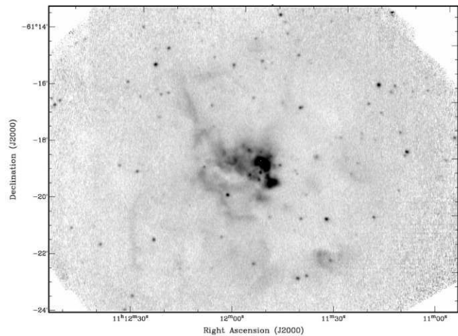
Fig. 1. SPIREX L-band ( 3.5 \mu\text{m} ) image of RCW 57. Total on-source integration of 60 minutes; effective resolution 2.6'' ; pixel scale 0.6'' ; 90% completeness limit at 11.2 mag; faintest star detected 13.5 mag.
