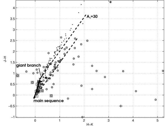
Fig. 8. JHK_s colour-colour diagram for RCW 57. The same symbols as in Figure 7 are used. The giant branch extends from (H-K_s)=0.13 to 0.31 with the same values for (J-H) as in the previous figure. The cross in the lower right corner indicates the mean error for all stars. The diagram shows the same sources as in the JHK_sL diagram using only the JHK_s -band data. Here the stars are clearly less separated than sources with IR-excess compared to using the L-band data. In this diagram only 25 sources would be classified as having IR-excess, compared to 75 in Figure 7, leading to an underestimate of the cluster disk fraction.
