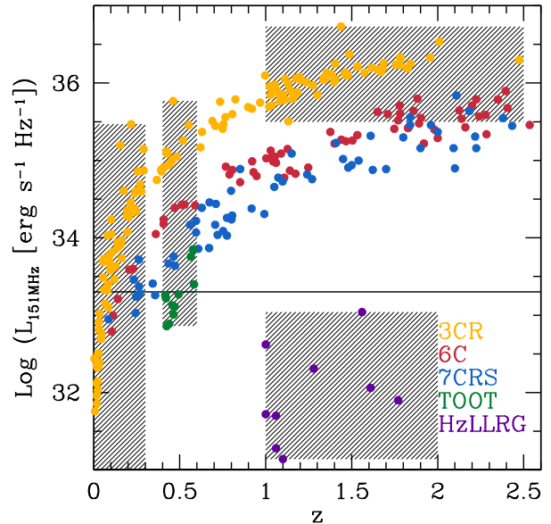
FIG. 1.— Radio loud samples considered in this paper. The horizontal line represents the canonical separation between low and high power radio galaxies (i.e. FR I and FR II, respectively). The color code identifies the different catalogs, and the shaded area show the regions of the radio luminosity v redshift plane where HST observations are suitable for this paper (see text). Here, the z < 0.3 range is covered by the 3CR sources (yellow), and the four groups that are part of the Willott sample (6C, 7C and TOOT are in red, blue and green, respectively plus the 3CR with z \sim 0.5 ) cover the range around z=0.5 . Both the low- z 3CR and the Willott sample are described in Sect. 4.1. The z > 1 range is covered again by the 3CR at high luminosity, and by the ECDFS HzLLRGs (purple) at the lowest luminosities. See Sect. 2 for more details.
