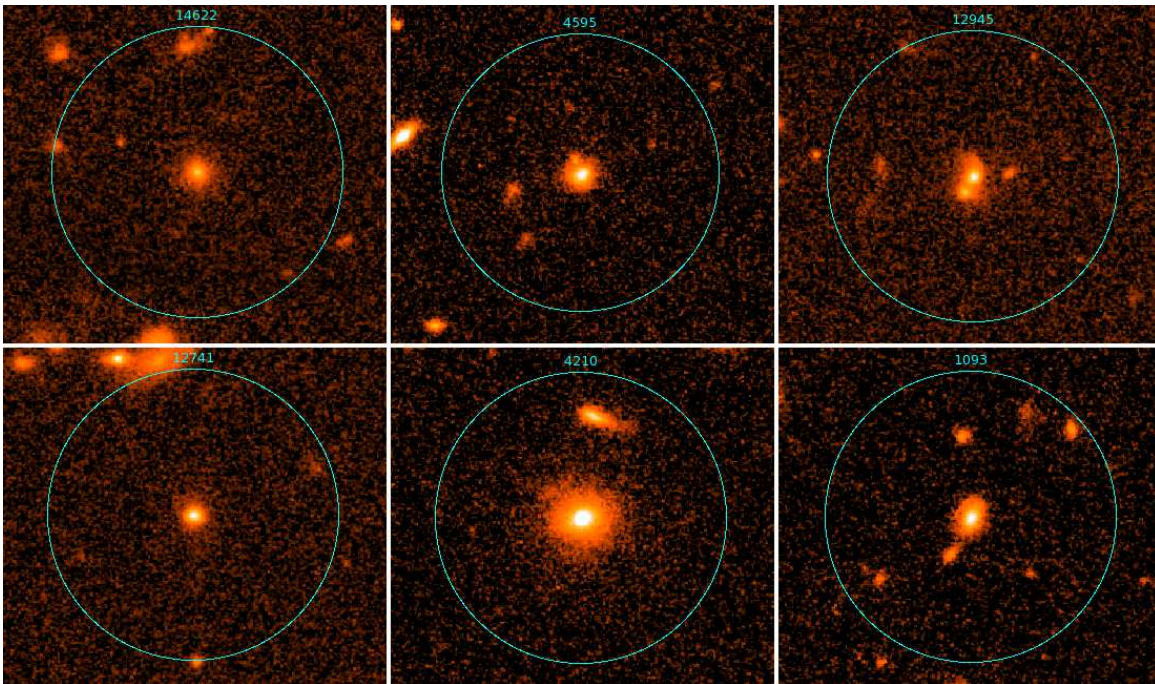
FIG. 4.— Six examples of non-active galaxies from our z > 1 sample. Both in the top and bottom rows, objects that are unanimously classified as non-mergers or mergers are shown in the left and right panels, respectively. Objects with mixed classification are shown in the middle panels. The circles are 6 arcsec radius, which correspond to \sim 50 kpc at the redshift of the objects. Images are from 3D-HST (Giavalisco et al. 2004; Brammer et al. 2012; Skelton et al. 2014, HST/WFC3/F140W)
