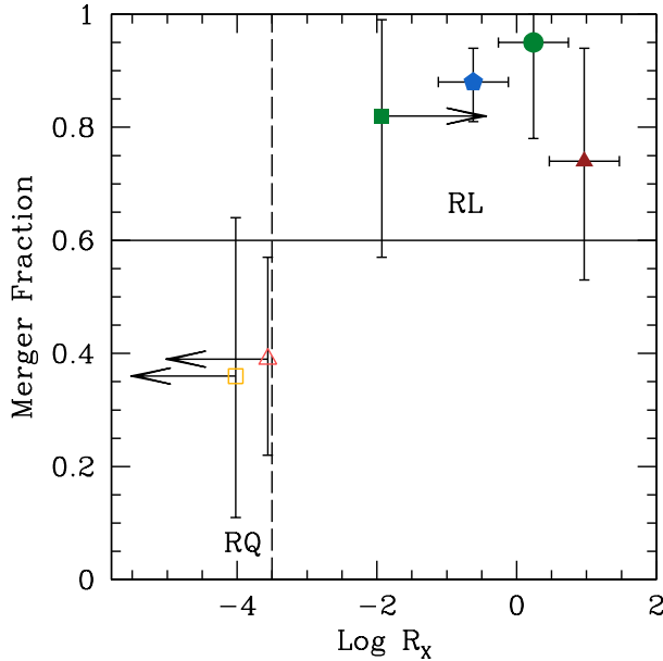
FIG. 6.— Merger fraction vs. average radio loudness parameter R_x for the different AGN samples. Filled symbols are the radio loud samples, empty symbols are radio quiet. The Hz3C sample is plotted as a circle, the HzLLRG is the square (lower limit), Willott's 3CRR is the triangle, and the low- z 3CR is the pentagon. For the radio quiet samples (empty symbols) the LPTy2AGN sample is the triangle, and the HPTy2AGN is the square. The dashed line represents the radio loudness threshold for PG QSOs (Terashima & Wilson 2003). The solid line marks the 60% merger fraction that appears to roughly separate radio-loud and radio-quiet samples. Color code is the same as for Fig. 5
