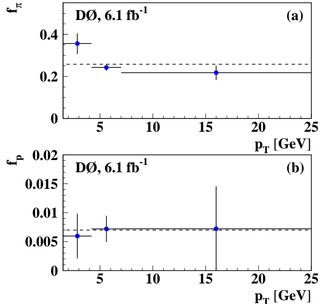
FIG. 6: The fraction of (a) \pi \rightarrow \mu tracks and (b) p \rightarrow \mu tracks in the inclusive muon sample as a function of the track transverse momentum. The horizontal dashed lines show the mean values of these fractions.
