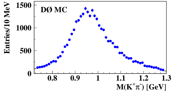
FIG. 24: The “ K^+\pi^- ” invariant mass distribution of simulated \rho^0 \rightarrow \pi^+\pi^- decays, where the mass of the charged kaon is assigned to one of the two reconstructed tracks.
