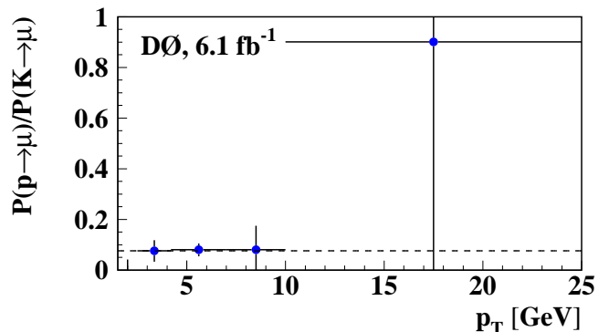
FIG. 4: The ratio P(p \rightarrow \mu)/P(K \rightarrow \mu) as a function of the particle transverse momentum. The horizontal dashed line shows the mean value of this ratio.
