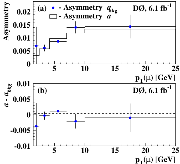
FIG. 14: (a) The asymmetry a_{\text{bkg}} (points with error bars) as expected from our measurements of the fractions and asymmetries of the background processes is compared to the measured asymmetry a of the inclusive muon sample (shown as histogram, since the statistical uncertainties are negligible). The asymmetry from CP violation is negligible compared to the background in the inclusive muon sample; (b) the difference a - a_{\text{bkg}} . The horizontal dashed line shows the mean value of this difference.
