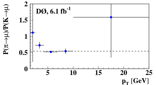
FIG. 3: The ratio P(\pi \rightarrow \mu)/P(K \rightarrow \mu) as a function of the hadron transverse momentum. The horizontal dashed line shows the mean value of this ratio.
