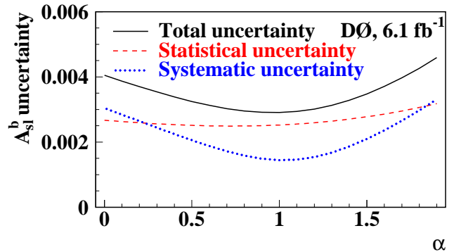
FIG. 15: Statistical (dashed line), systematic (dotted line), and total (full line) uncertainties on A_{\text{sl}}^b as a function of the parameter \alpha of Eq. (64).
